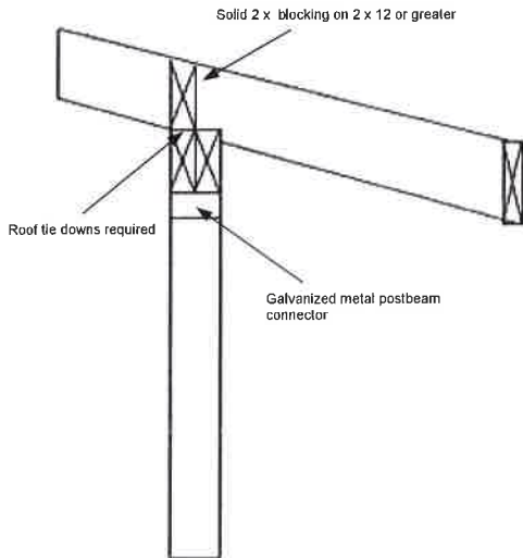
Standard Post Attachment
