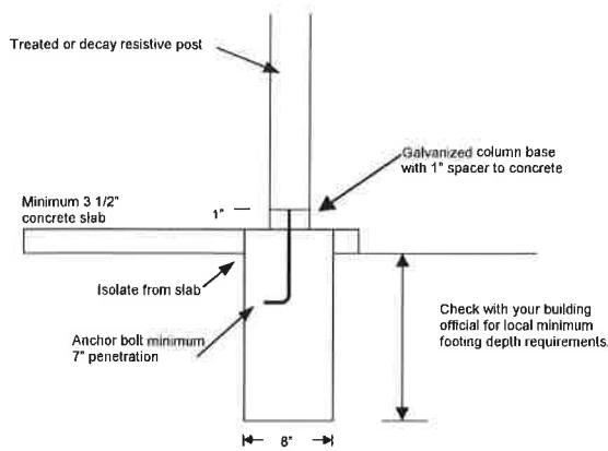
Standard Footing Detail
